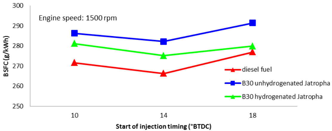
Figure 2. BSFC at engine speed 1,500 rpm
