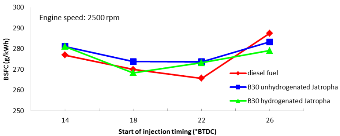
Figure 3. BSFC at engine speed 2,500 rpm
