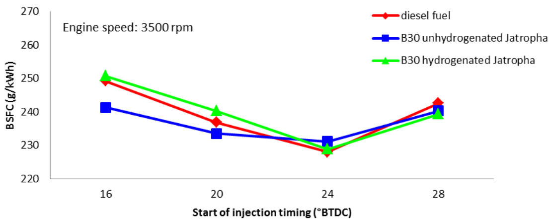
Figure 4. BSFC at engine speed 3,500 rpm
