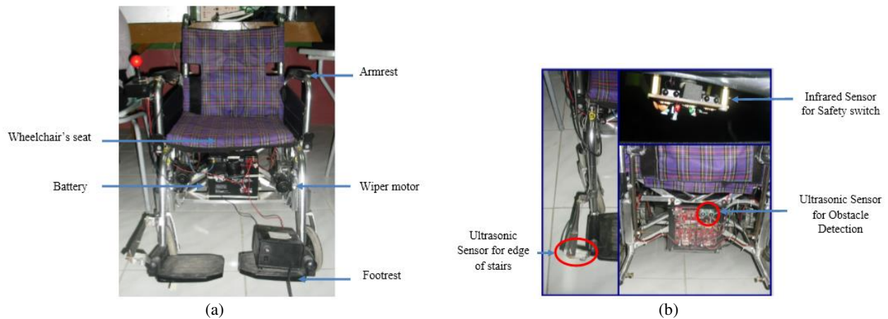
Figure 4. The developed electronic wheelchair; (a) front view; (b) back view
