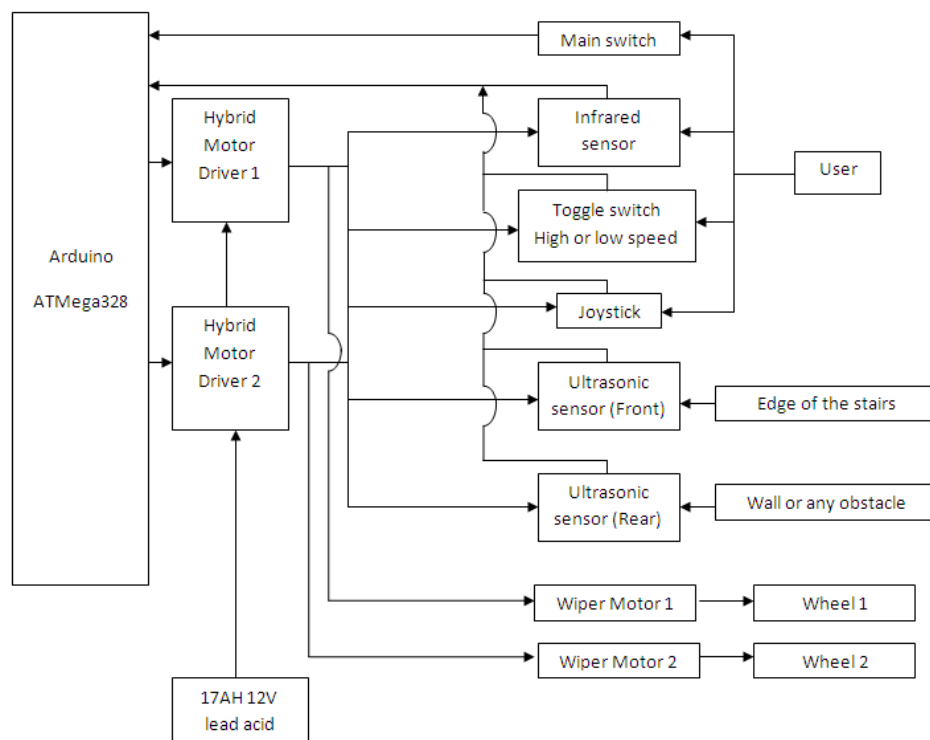
Figure 2. Block diagram of the designed low-cost electronic wheelchair
