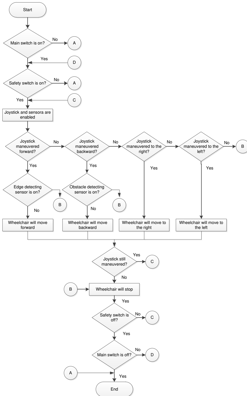
Figure 5. The system flowchart
