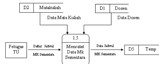
Gambar 4.7 DFD Level 1 Temp
