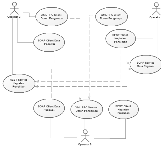
Gambar. 9. Diagram Use Case Model Integrasi Data
