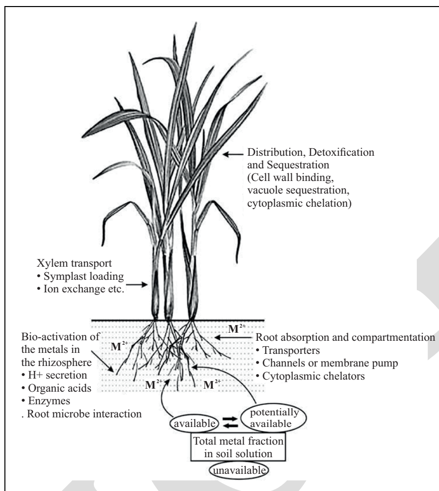
Figure 2. General mechanism of metal hyperaccumulation by plants.
