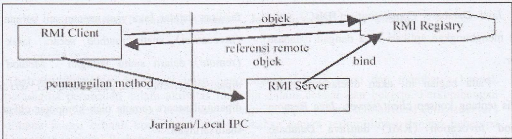
Gambar 1. Mekanisme Kerja Remote Method Invocation (RMI)
