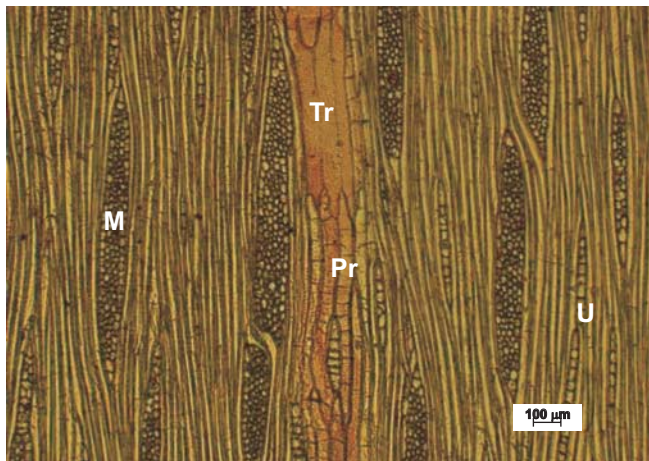
Figure 4. Tangential section of Shorea mujongensis wood
