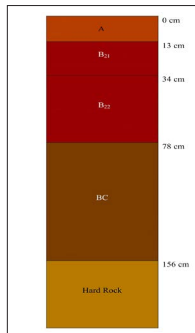
Figure 2. Profile of a limestone sequence in Hitu.
