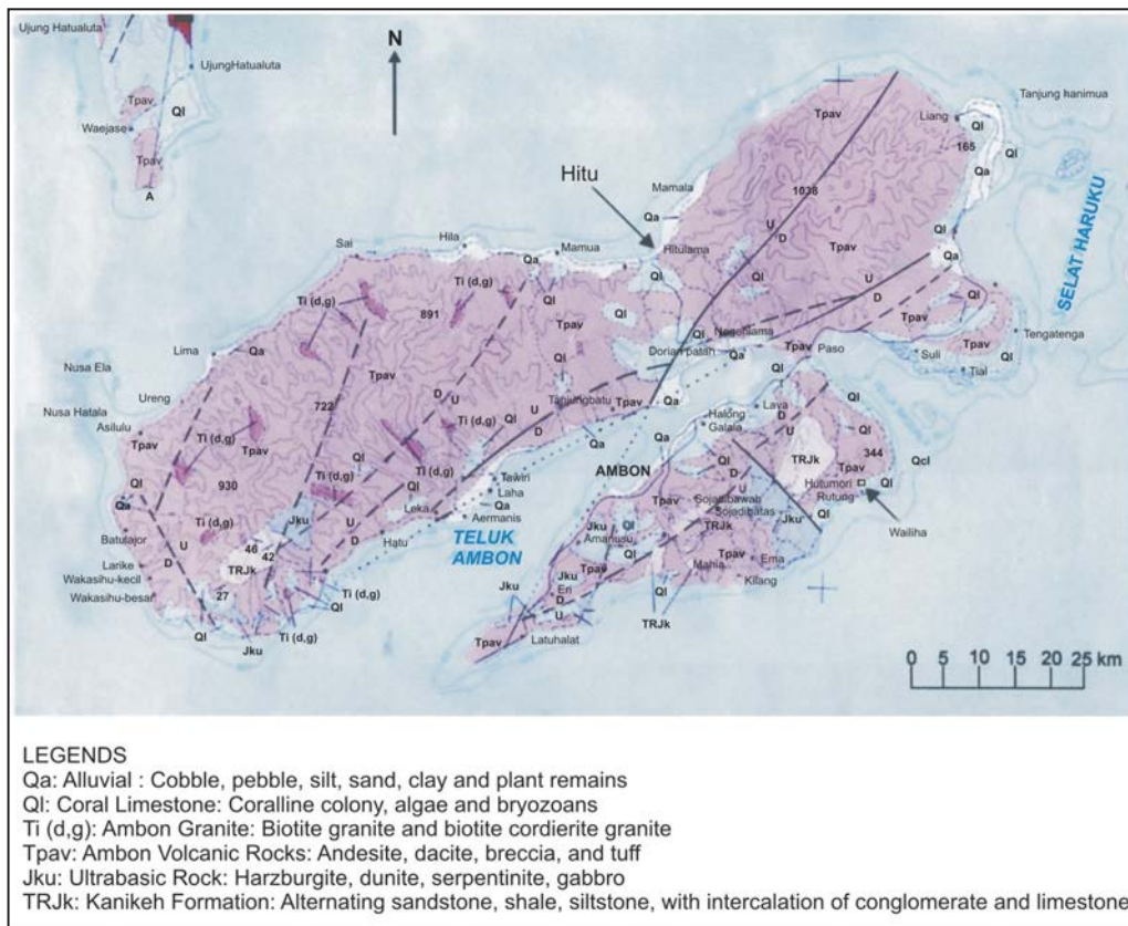
Figure 1. Locality and geological map of the studied profile (geological map after Tjokrosapoetro et al. , 1994).
