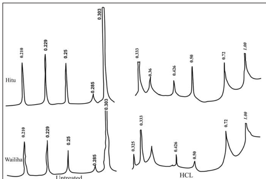
Figure 4. XRD patterns of untreated and HCL treated of rock fragments of the studied profiles.
