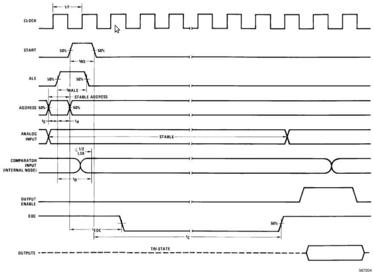
Gambar 4. Timing Diagram ADC0808, [5]
