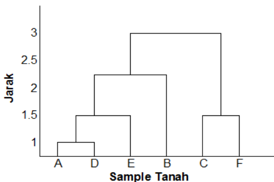
Gambar 1. Dendogram Clustering
