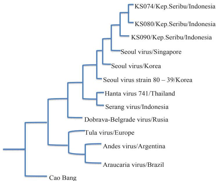
Figure 3. Phylogenetic tree of Indonesia viruses found in Kepulauan Seribu Phylogenetic tree was generated by Mega 5 software; Cladogram UPGMA analysis of S gene nucleotide Seoul virus traces of three strains of virus found in the Kepulauan Seribu in 2009 by Hantavirus species S gene from other countries.
