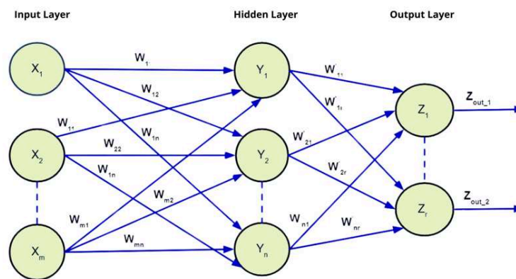
Gambar 4. Proses Learning Jaringan Neural
