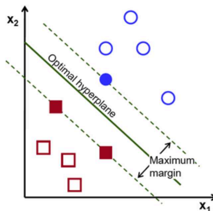
Gambar 3. Hyperplane Support Vector Machine (SVM) [16]
