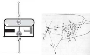
Figure 4. COG-COB Orientation on Vehicle [12-13]
