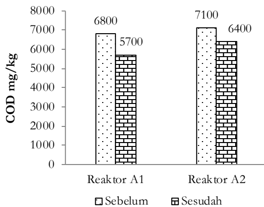
Gambar 2. Nilai COD slurry
