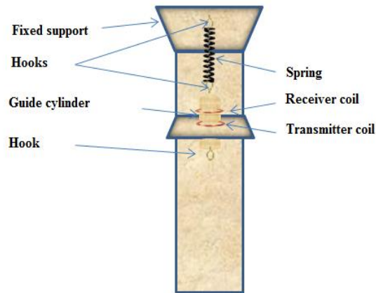
Figure 1. Electromagnetic Sensor
