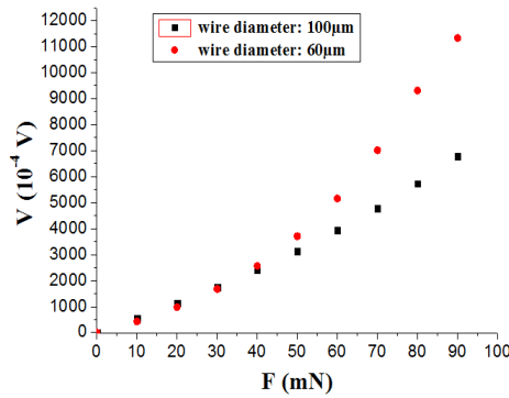
Figure. 3. Sensor response for different wire diameters
