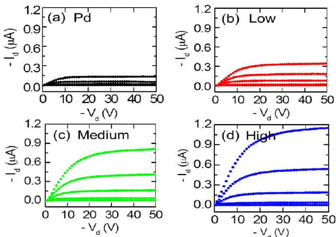
Figure 4. Output characteristics ( I_d - V_d ) of pentacene transistors at V_g = 0, -5, -10, -15 and -20 V (bottom to top) for (a) zero, (b) low, (c) medium, and (d) high density SWCNT in the electrodes.
