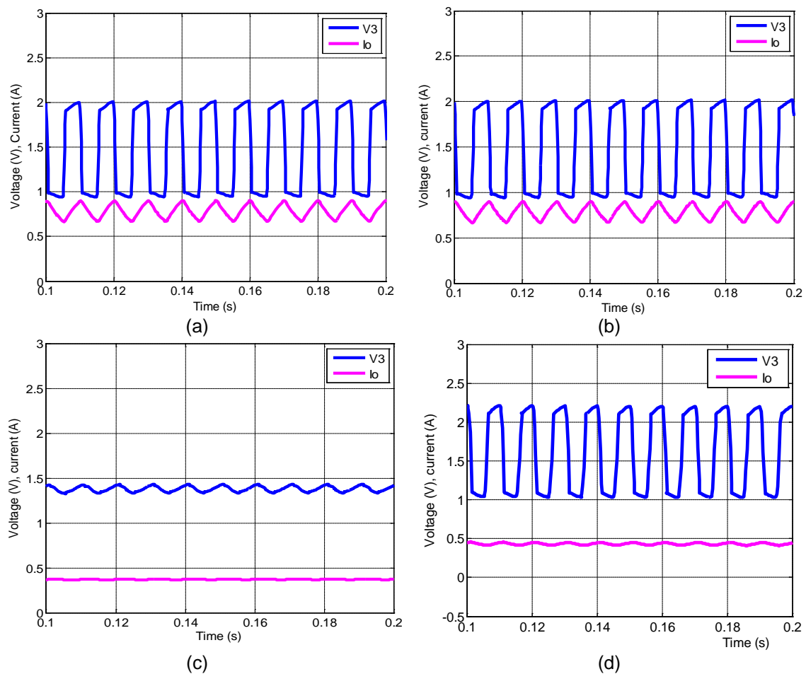
Figure 7. Output voltage V_3 and output current waveforms
