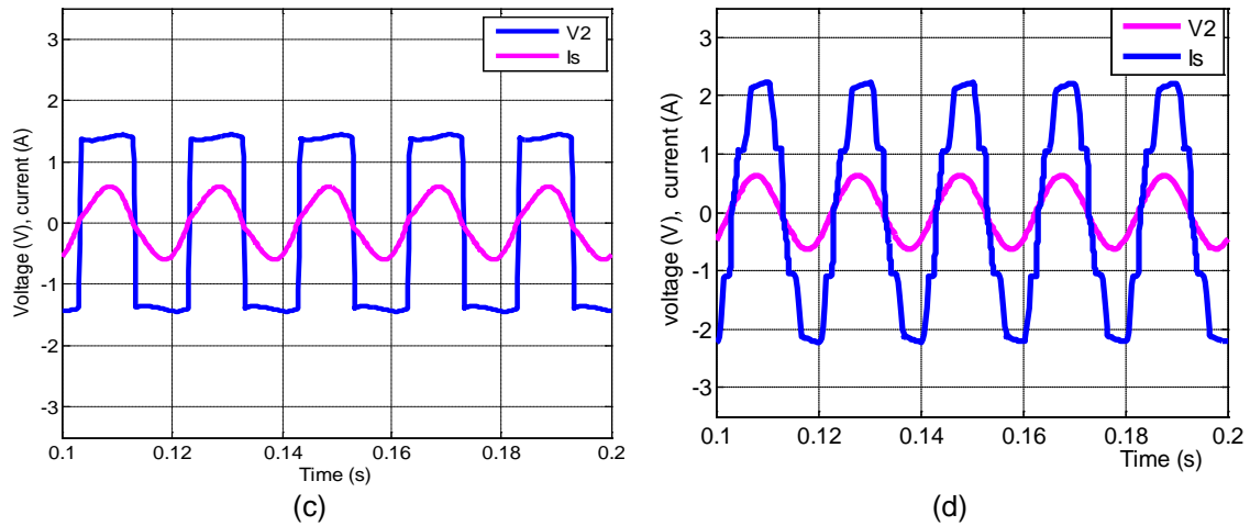
Figure 6. Input voltage V_2 and input current waveforms
