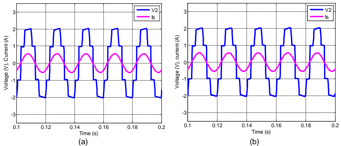
Figure 5. Input voltage and input current waveforms
