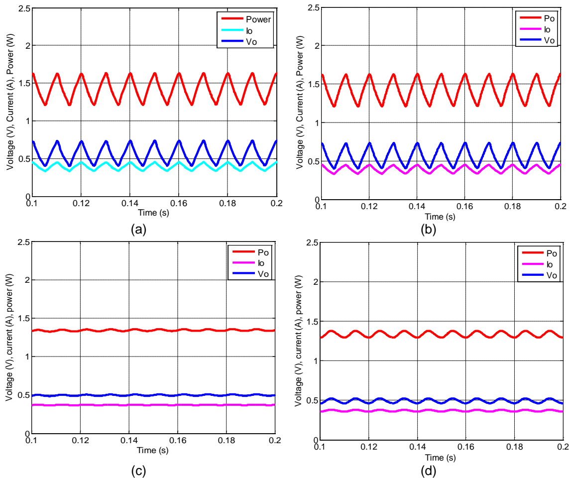
Figure 8. Output voltage, current and power waveforms
