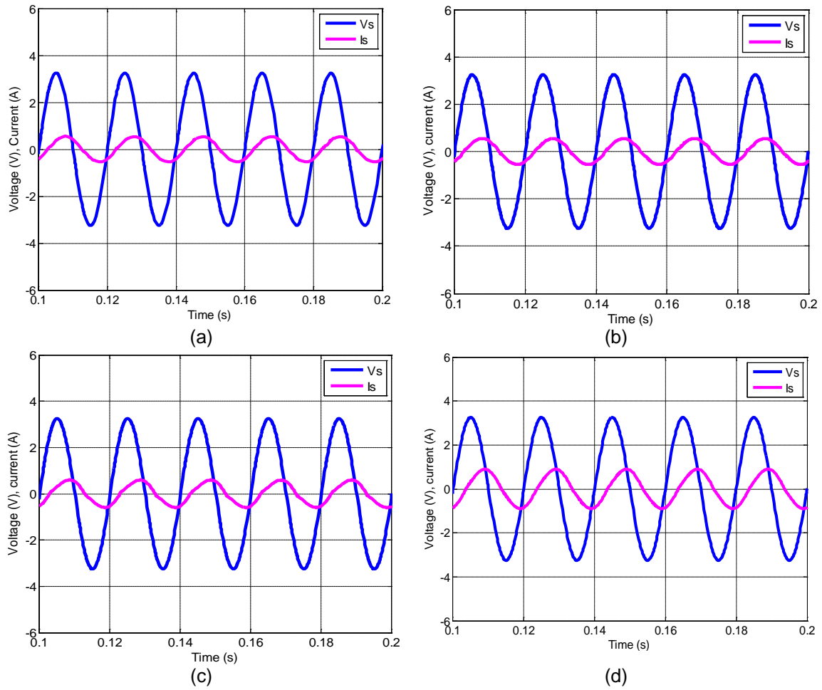
Figure 5. Input voltage and input current waveforms
