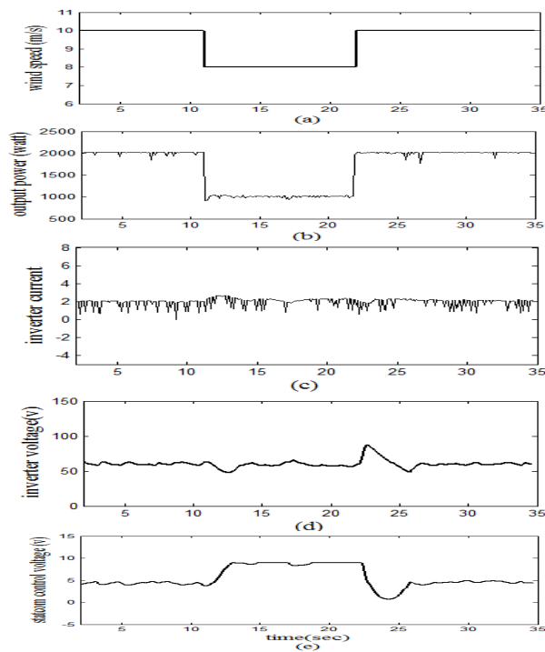
Figure 12. Experimental voltage regulation of wind system at step up-down-up in wind speed using PI controller
