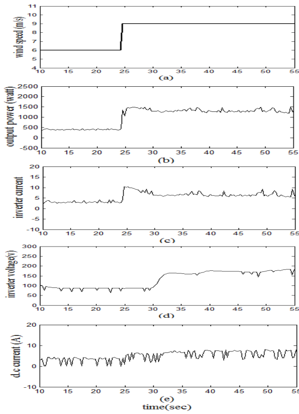
Figure 6. Wind turbine performance with inverter at step up in wind speed
