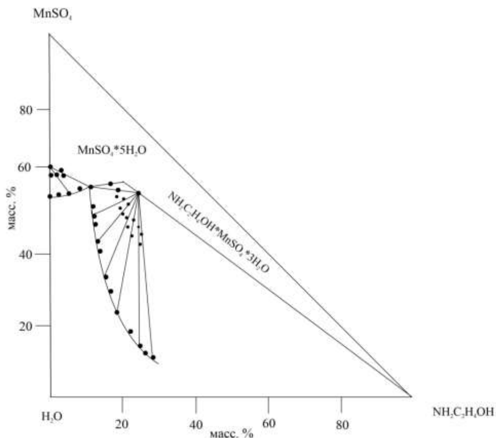
Rice. 1. Andzotherm solubility system manganese sulfate - monoethanolamine - water at 10°C.
