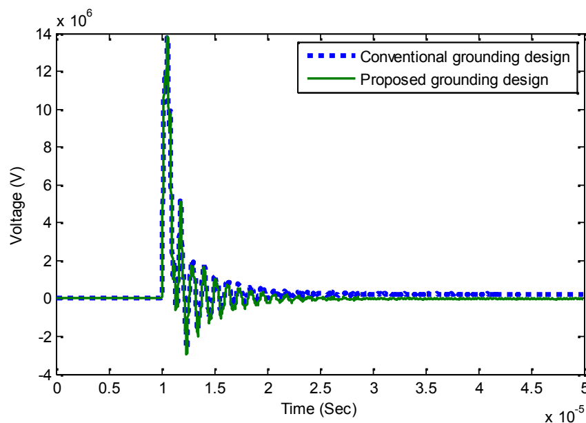
Figure 10. Tower top voltage under only 51kA 2/631 s
