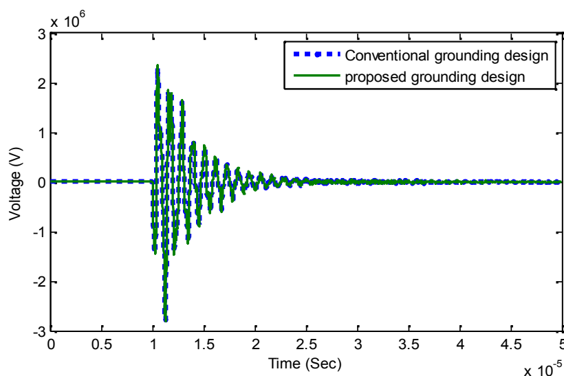
Figure 5. Insulation layer voltage under only 51kA 2/631 s
