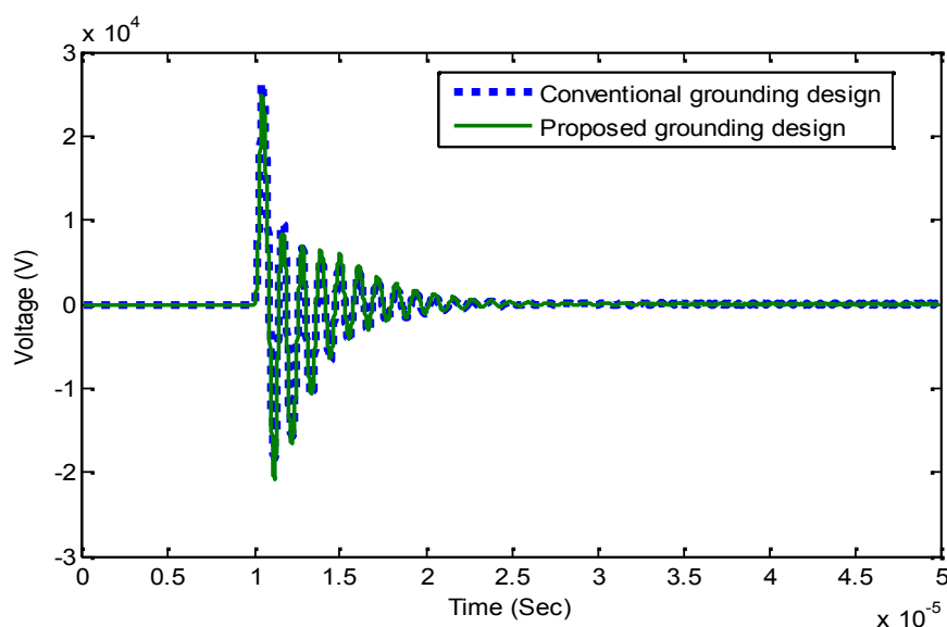
Figure 7. Control device voltage under only 51kA 8/20 s
