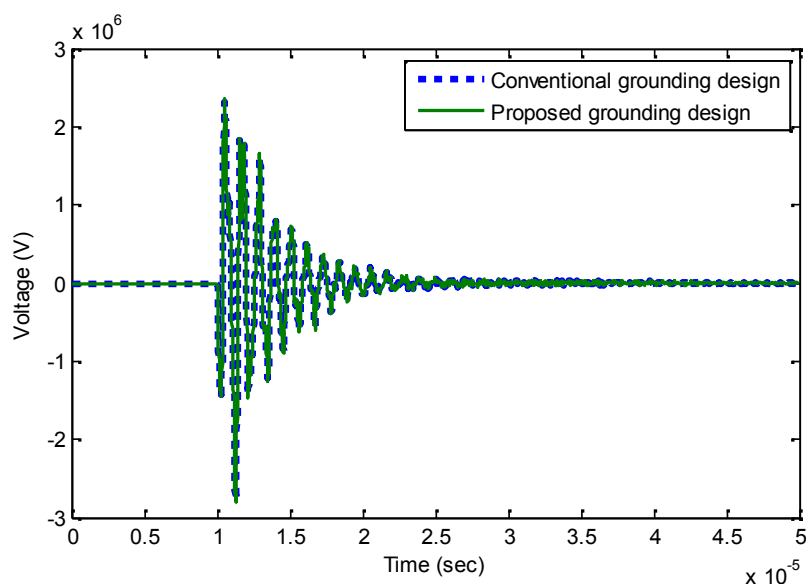
Figure 4. Insulation layer voltage under only 51kA 8/20 s
