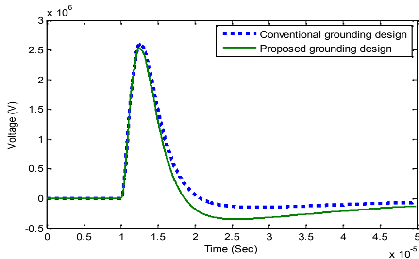
Figure 9. Tower top voltage under only 51kA 8/20 s
