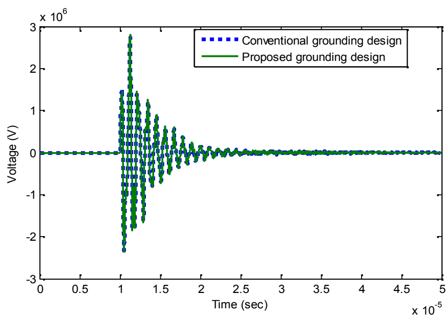
Figure 8. Control device voltage under only 51kA 2/631 s
