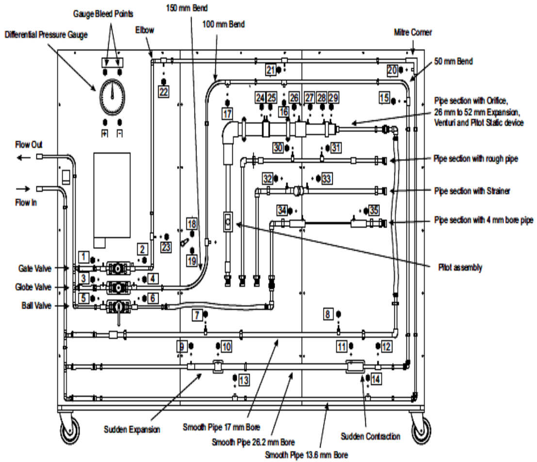
Figure 1. Experimental schematic diagram [10]
