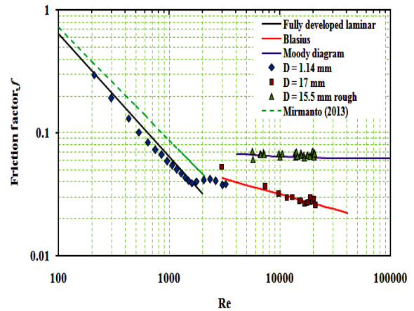
Figure 5. Experimental friction factors
