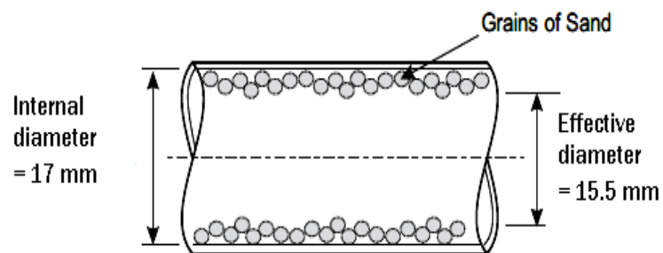
Figure 2. Rough pipe test section
