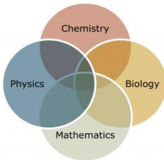
Figure 1. Venn diagram showing the interconnections between natural sciences.
