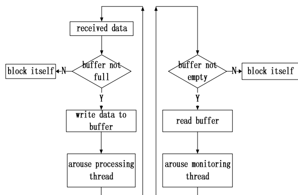
Figure 4. Monitoring and processing flow chart
