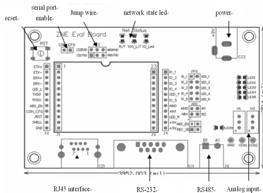
Figure 3. ZNE-100TL circuit diagram
