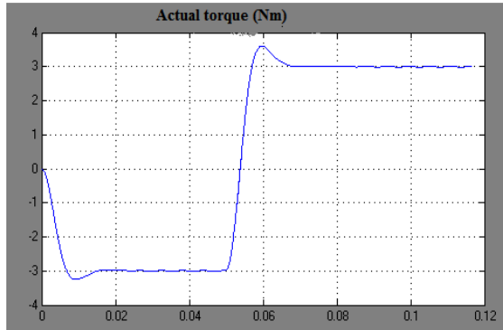
Figure 12. Electromagnetic Torque ( T_{e\_Nm} ) of the PMSM.
