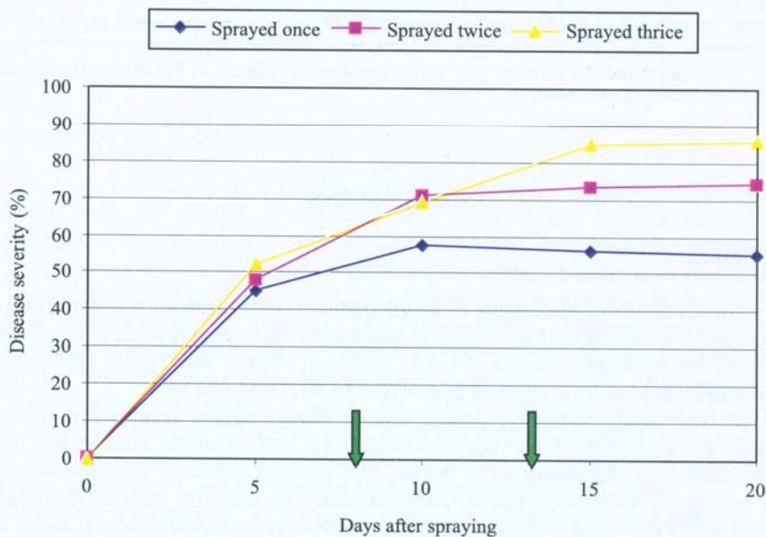
Figure 1. Disease severity (%) of Exserohilum leaf blight on a highly susceptible ecotype (PK-04) caused by E. longirostratum . The arrows indicate the days when double and triple applications were administered.
