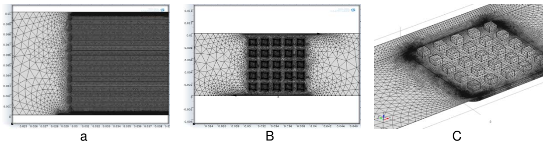
Figure 5. 1D, 2D and 3D Fine Mesh Generation at Fin Assembly was Shown in a, b and c Respectively
