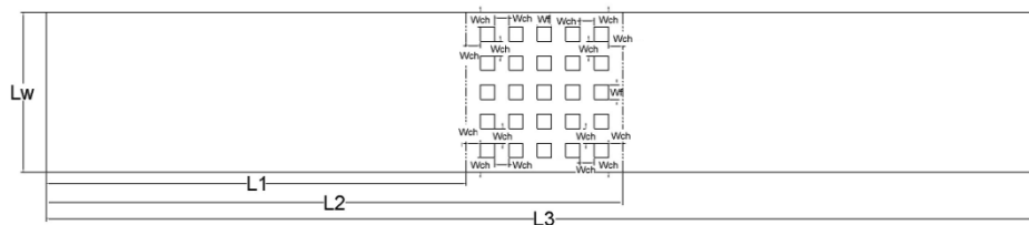
Figure 3. A Schematic of Micro-channel Cooling Assembly with Micro-fin Array Architecture, 2D Fin Array, M=5 , N=5
