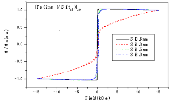
Fig. 2. Magnetization curve of [\text{Fe}(2\text{nm})/\text{Si}(t_{\text{Si}})]_{30} MLs at RT.
