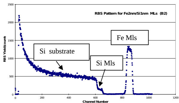
Fig. 6. Rutherford Back Scattering pattern of [Fe(2nm)/Si(1nm)]_{30} MLs.
