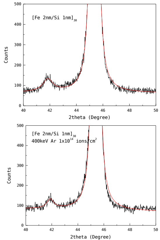
Fig. 5. X ray diffraction pattern of Fe(2nm)/Si(1nm) MLs for as deposited sample (upper), and post 400keV Argon ion irradiation at dose 1 \times 10^{14} ion/cm 2 (lower).
