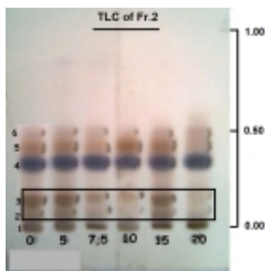
Fig. 2. TLC of fraction 2 from ethyl acetate extracts of irradiated and unirradiated tea parasite herbs (condition: silica gel GF 254 , n-hexane - ethyl acetate (3:1), UV light at 254 nm, 1% cerium sulphate in 10% sulfuric acid).
