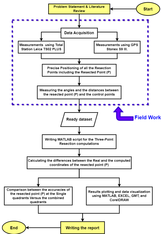
Figure 2. Flowchart of the investigation strategy for the three-point resection method accuracy.
