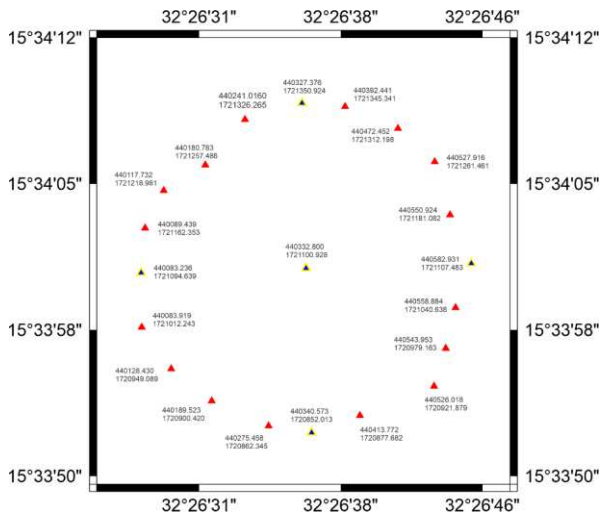
Figure B1. The coordinates of the resection points.
