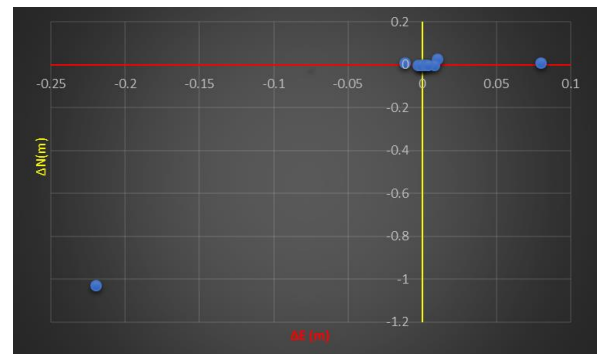
Figure 7. The accuracy of the resected point (P) in the second quadrant.
