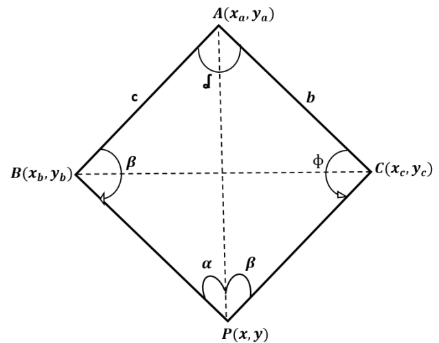
Figure 4. The positions of resected point P and control points (A, B, and C) [7].
