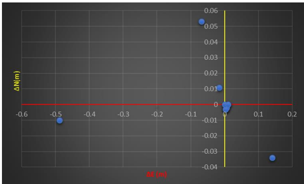
Figure 13. The accuracy of the resected point (P) at the combination of the fourth and first quadrants.
