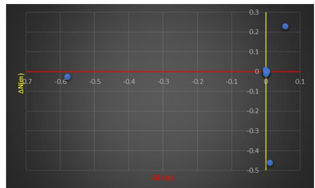
Figure 12. The accuracy of the resected point (P) at the combination of the third and fourth quadrants.
