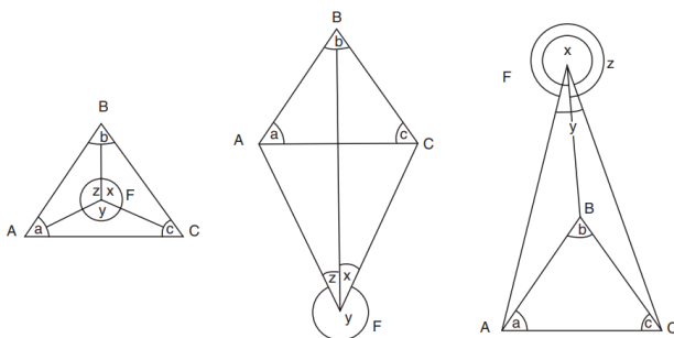
Figure 3. The three cases of the angular resection [18].
