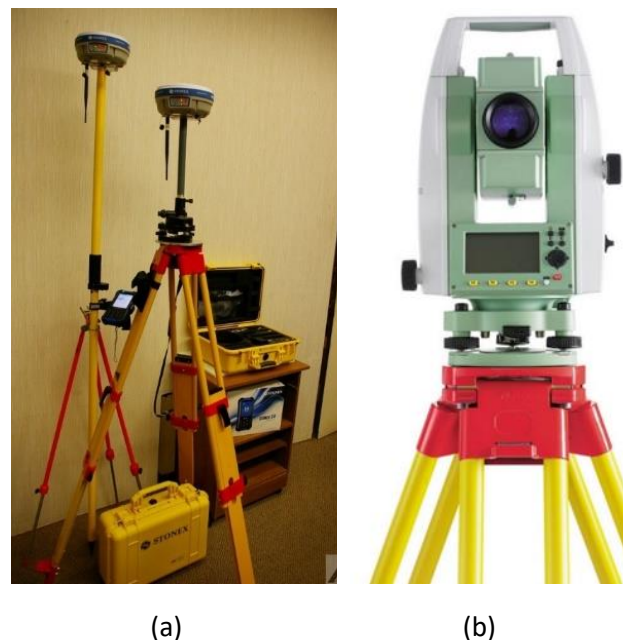
Figure 1. Instruments used in the surveying works (a) GPS Stonex S9 III. (b) Total Station Leica TS02 PLUS.
