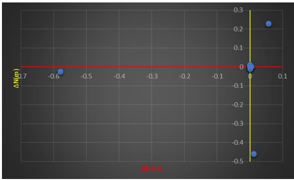
Figure 8. The accuracy of the resected point (P) in the third quadrant.
