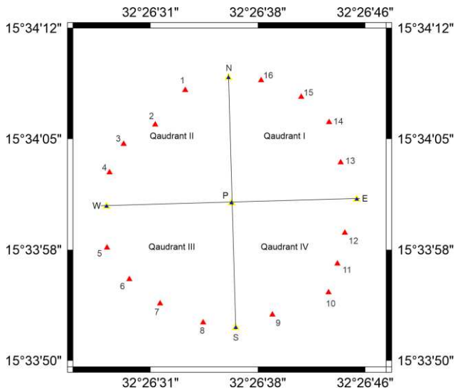
Figure 5. Distribution of the control points around the resected point across four-quadrants.
