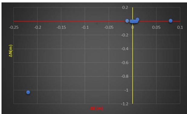
Figure 11. The accuracy of the resected point (P) at the combination of the second and third quadrants.
