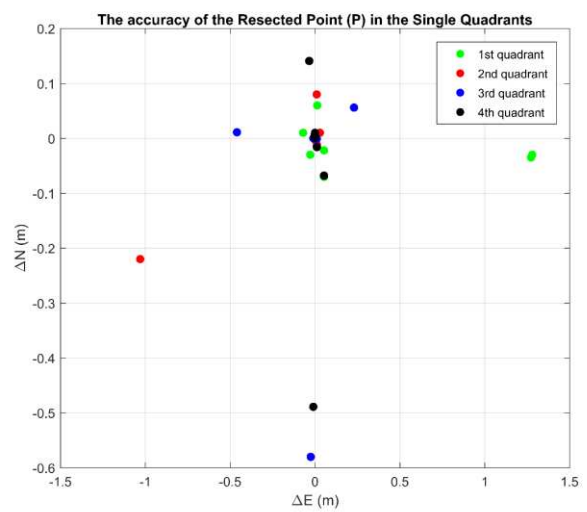
Figure A1. The accuracy of the resected point (P) at the single quadrants.
