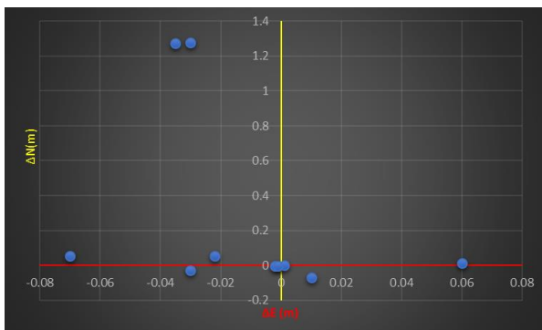
Figure 6. The accuracy of the resected point (P) in the first quadrant.
