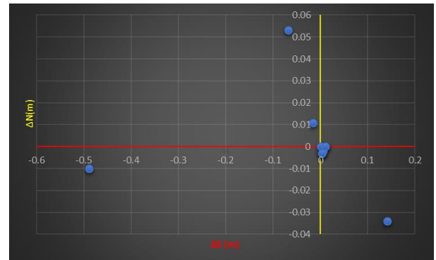
Figure 9. The accuracy of the resected point (P) in the fourth quadrant.
