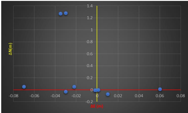
Figure 10. The accuracy of the resected point (P) at the combination of the first and second quadrants.
