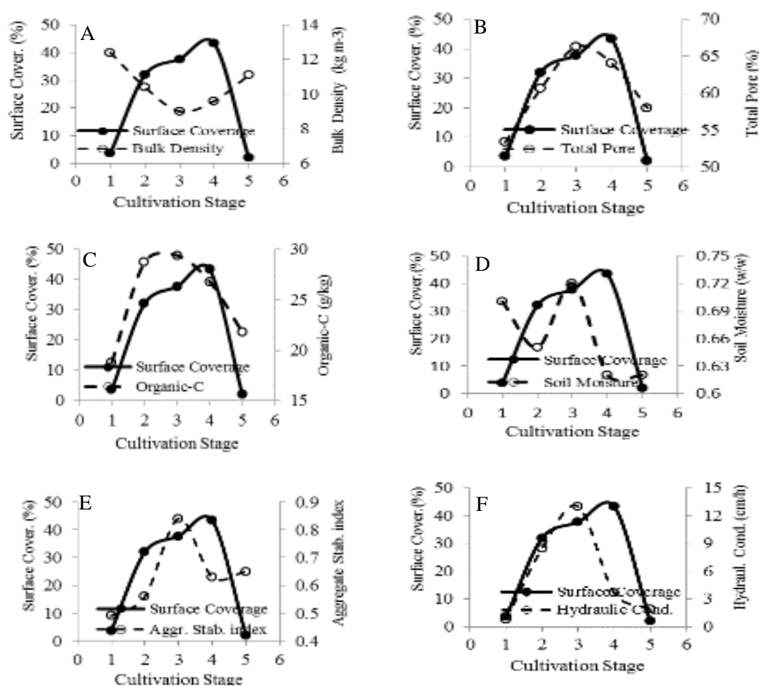
Figure 2. The effect of surface coverage on soil Bulk Density (A), Total Pore (B), Organic-C (C), Soil Moisture (D), Aggregate Stability Index (E), and Hydraulic Conductivity (F) of Ultisol Limau Manis during soybean cultivation
