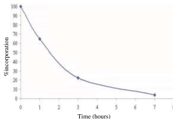
Fig. 4. Viability of LAB in the small intestine of catfish as determined by using the 32 P radioisotope.
