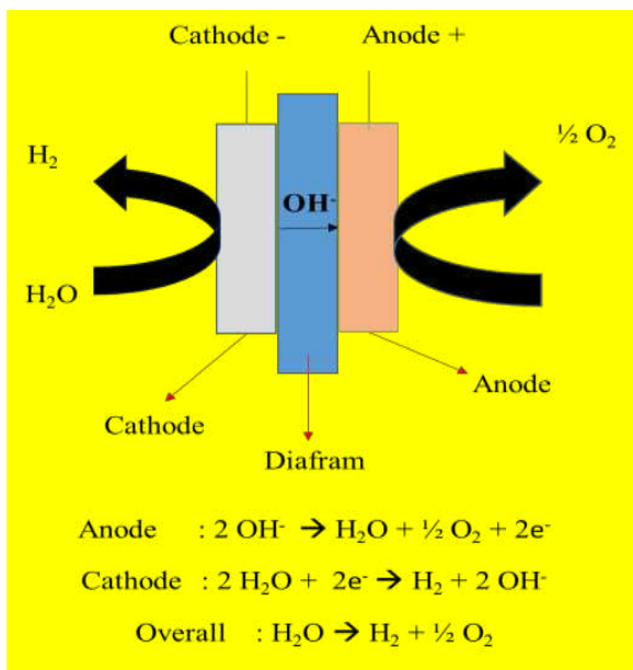
Figure 1. Electrolysis reaction of water
