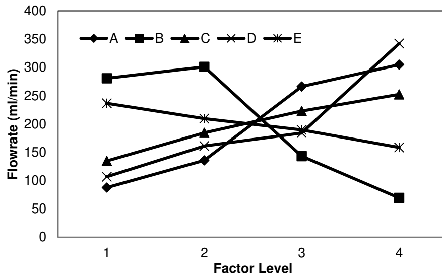
Figure 10. The plot of the mean response of HHO flowrate
