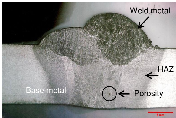
Figure 2. Macrostructure photo without WPS
