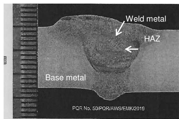
Figure 3. Macrostructure photo with WPS
