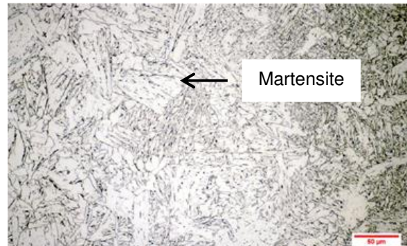
Figure 5. Microstructure at HAZ without WPS
