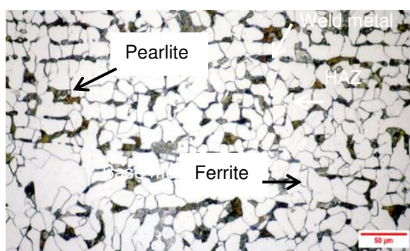
Figure 4. Microstructure photos of base metal
