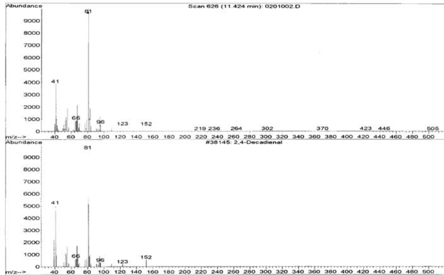
Figure 3. GCMS spectrum and fragmentation pattern of A) isolated compound of Jatropha curcas and B). 2,4-decadienal
