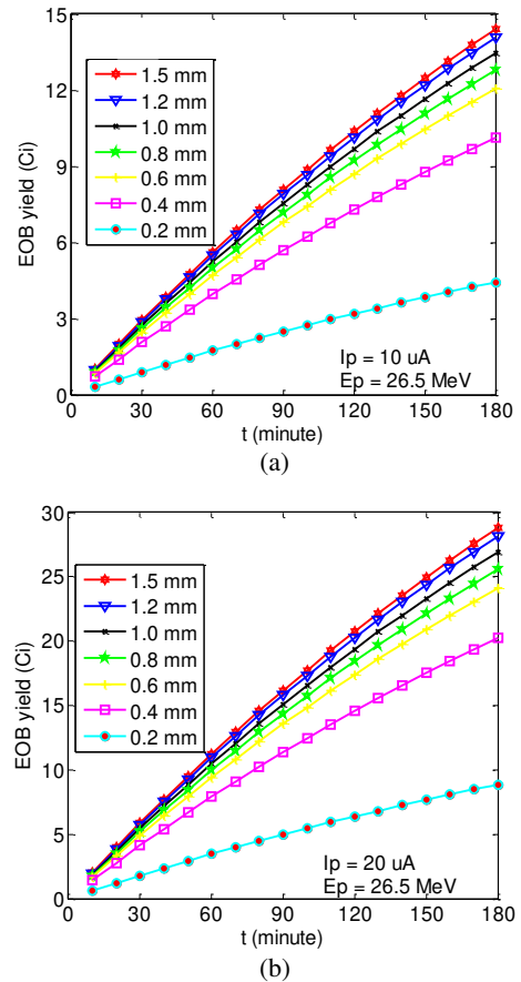
Fig. 3. EOB yields as a function of irradiation time at different Ni target thickness and fixed energy of 26.5 MeV for proton beam current of (a) 10 μA, and (b) 20 μA.
