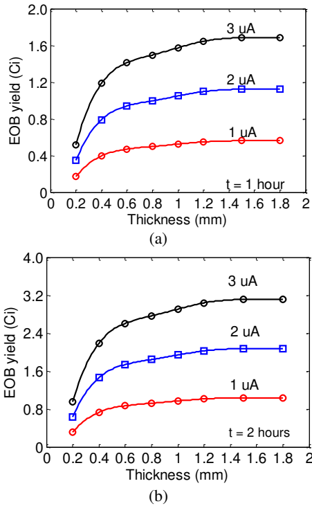
Fig. 2. EOB yields as a function of Ni target thickness at different proton beam current ranging from 1 μA to 3 μA and fixed energy of 26.5 MeV for irradiation time of (a) 1 hour and (b) 2 hours.
