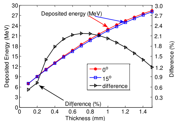
Fig. 1. SRIM-calculated proton deposited energy as a function of nickel target thickness.
