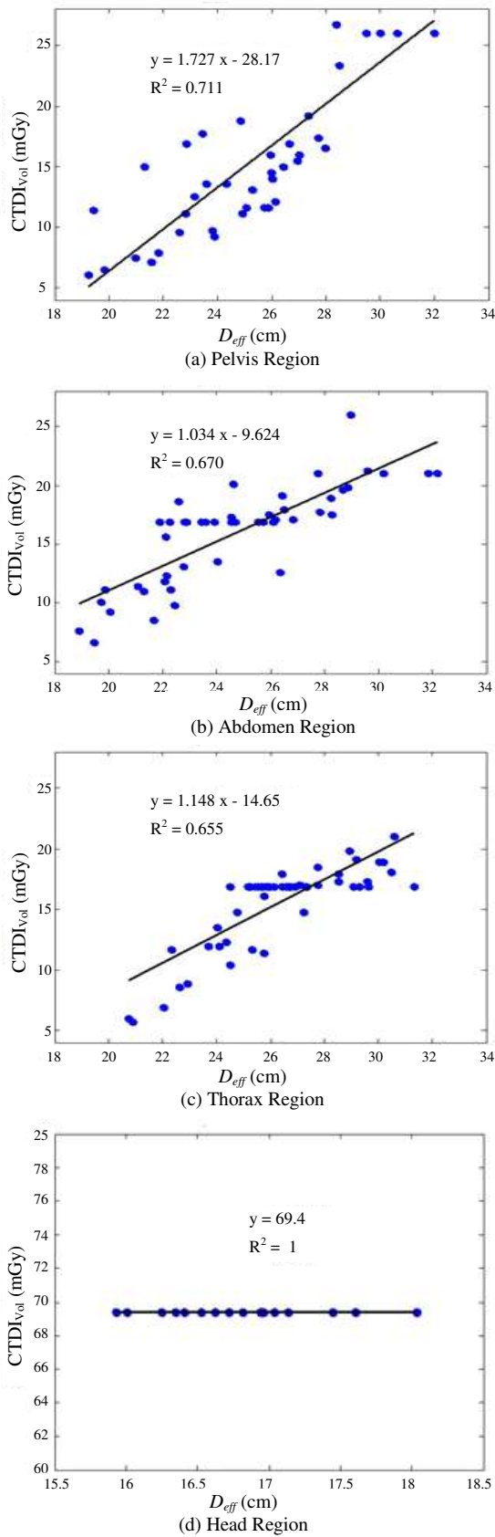
Fig. 2. The relationship between D_{eff,m} and CTDI_{vol} for pelvis (a), abdomen (b), thorax (c), and head examinations (d).
