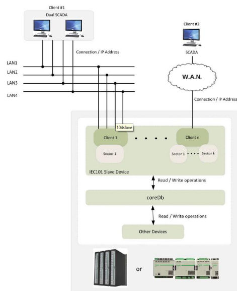
Gambar 2. Protocol IEC 104 Slave
