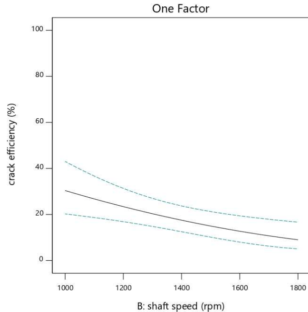
Fig. 6. Crack efficiency and shaft speed
