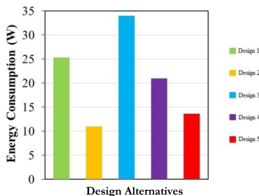
Figure 7. Comparison of Power Needed For Each Alternatives (P) (b)
