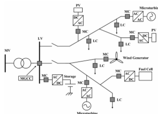
Figure 1. MG Architecture, Comprising MS Loads and Control Devices
