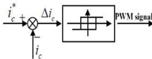
Figure 4. Hysteresis Current Control Visual Aid
