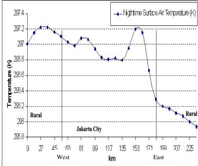
Figure 6. The MM5 modified land cover model of domain 3 for west-east vertical cross-section of simulated surface temperature (K) at 23.00 LST on August 6, 2004.
