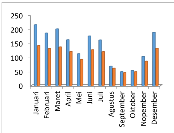
Figure 1. Calculation of Effective Rainfall and Rainfall 2010-2019
