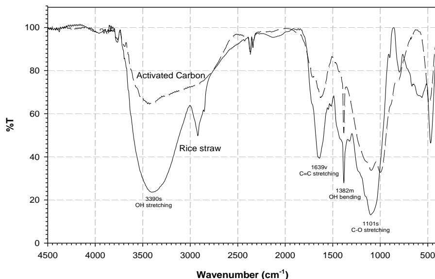
Figure 2. FTIR spectra of rice straw and its corresponding activated carbon.
