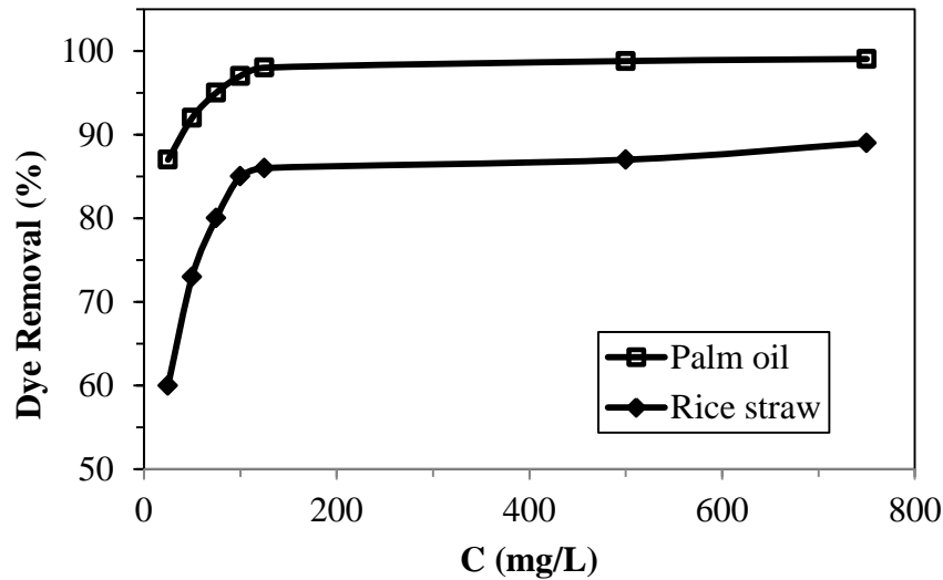
Figure 5. Adsorption isotherms of Naphtol AS-G adsorbed by activated carbon made from rice straw and palm oil midrib. Experimental conditions: equilibrium time = 60 minutes, adsorbent mass = 0.1 g, temperature = 25°C, pH = 5.0).
