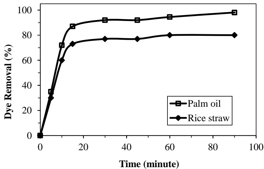
Figure 4. Effects of contact time on Naphtol AS-G adsorbed by activated carbon made from rice straw and palm oil midrib. Experimental conditions: dye concentration = 100 mg/L, adsorbent mass = 0.1 g, temperature = 25°C, pH = 5.0).
