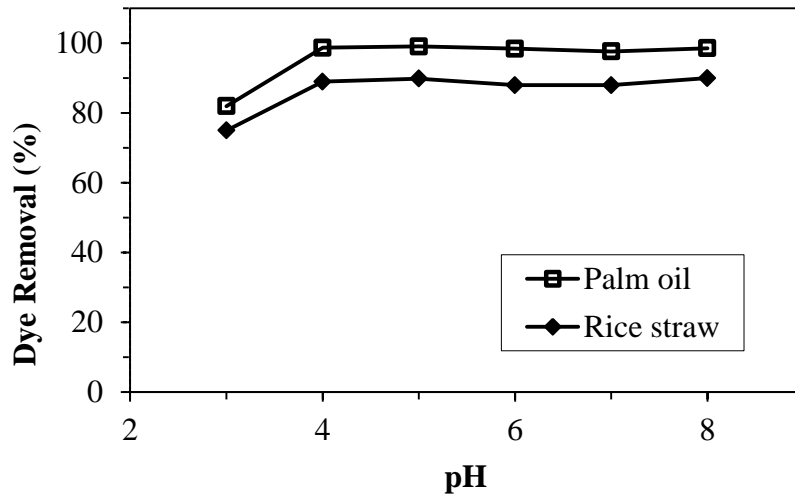
Figure 3. Effects of pH on Naphtol AS-G adsorbed by activated carbon made from rice straw and palm oil midrib. Experimental conditions: equilibrium time = 60 minutes, dye concentration = 100 mg/L, adsorbent mass = 0.1 g, temperature = 25°C).
