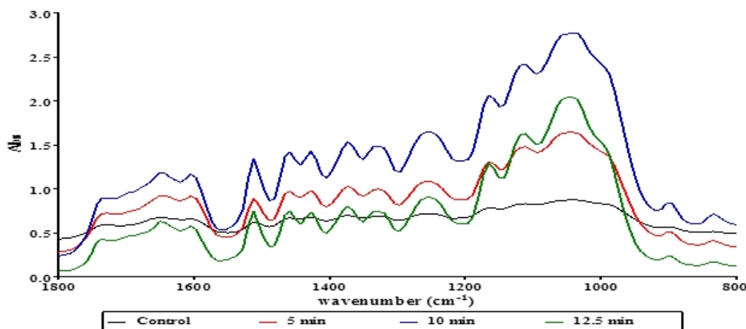
Figure 6 FTIR spectra of bamboo after biological pretreatment (5% inoculum loading for 30 days) subjected to microwave pretreatment (1) 1,736 cm -1 , (2) 1,512 cm -1 , (3) 1,373 cm -1 , (4) 1,165 cm -1 and (5) 897 cm -1
