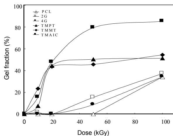
Fig. 4. Gel fraction dose curves of PCL containing 1% weight of different monomers.
