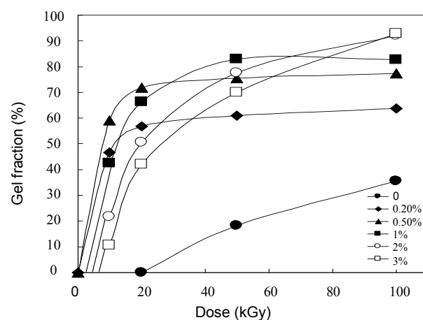
Fig. 7. Gel fraction-dose curves of PBSA with TMAIC in different concentrations.
