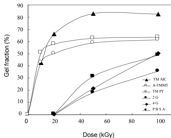
Fig. 5. Gel fraction-dose curves of PBSA containing 1% weight of different monomers.
