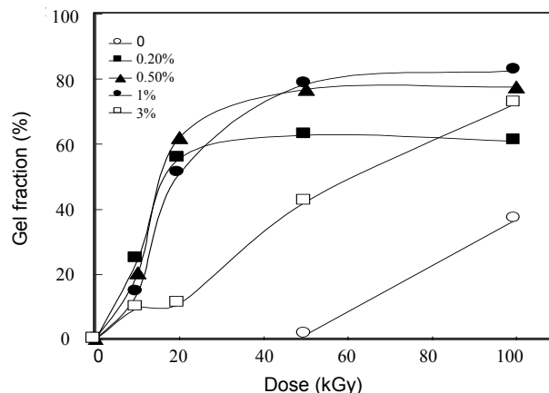
Fig. 6. Gel fraction-dose curves of PCL with TMAIC in different concentrations.
