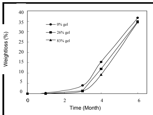
Fig. 11. Soil burial test of PBSA with different gel contents (pure PBSA (0% gel); irradiated PBSA (26% gel) irradiated at 50 kGy; irradiated PBSA containing 1% TMAIC (83% gel) irradiated at 50 kGy).
