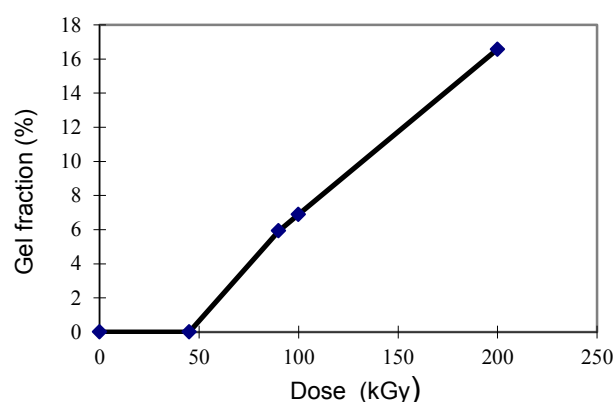
Fig. 3. Gel fraction dose curves of P4HB.
