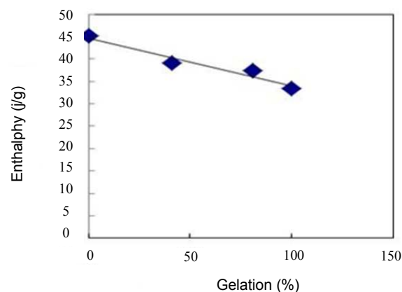
Fig. 10. Enthalpy-gel fraction curves for PBSA.
