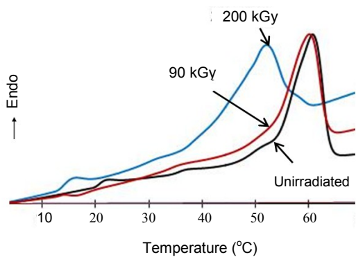
Fig. 8. Melting behaviors curves of irradiated P4HB.
