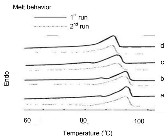
Fig. 9. Melting behaviors curves of irradiated PBS1 in the presence of 1% of TMAIC: (a) 0% gel fraction, (b) 43% gel fraction, (c) 83% gel fraction and (d) 100% gel fraction.
