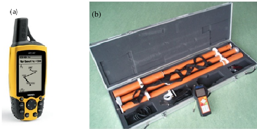
Figure 3. Survey equipments; (a) Global position system (b) Conductivity Multi-depth (CMD)-4 Electromagnetic Conductivity Meter.
