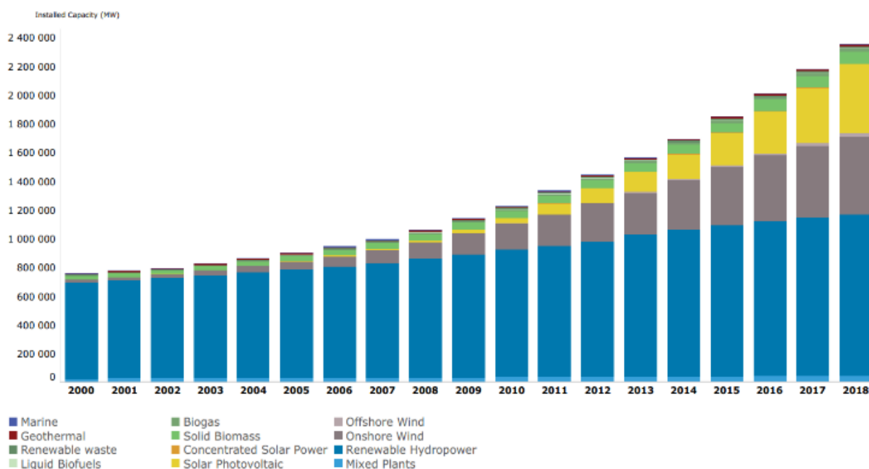
Figure 2. Global trend of increasing the capacity of renewable energy sources by type (IRENA))
