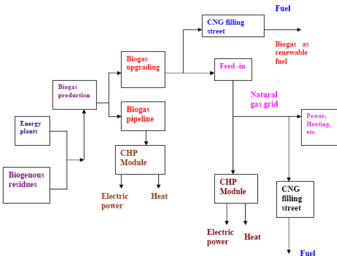
Figure 4. Overview of biogas utilisation pathways (Omer, 2008)
