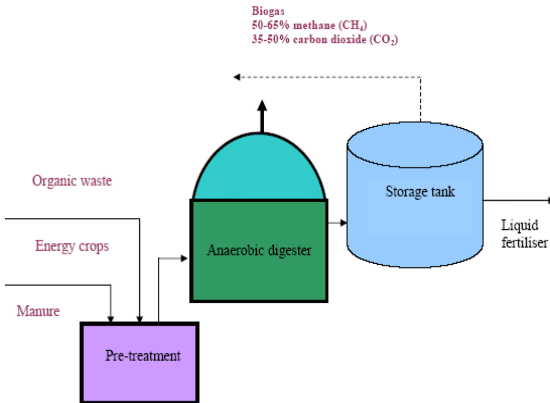
Figure 1. General schematic of an agricultural biogas plant (Omer, 2012)
