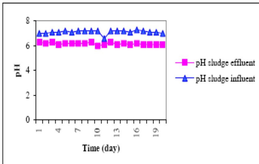
Figure 6. pH sludge before and after treatment in the digester
