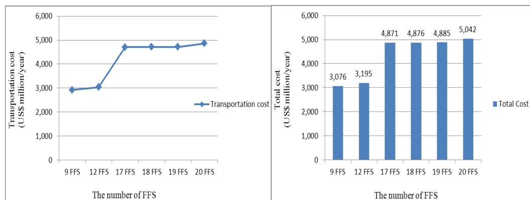
Figure 4c. number of FFS vs. transportation cost
