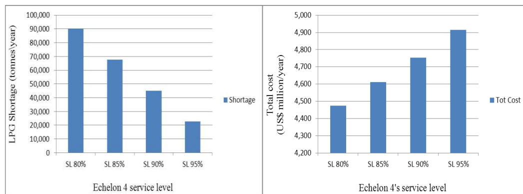
Figure 5a. service level vs. shortages
