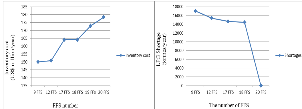
Figure 4a. Number of FFS vs. shortage
