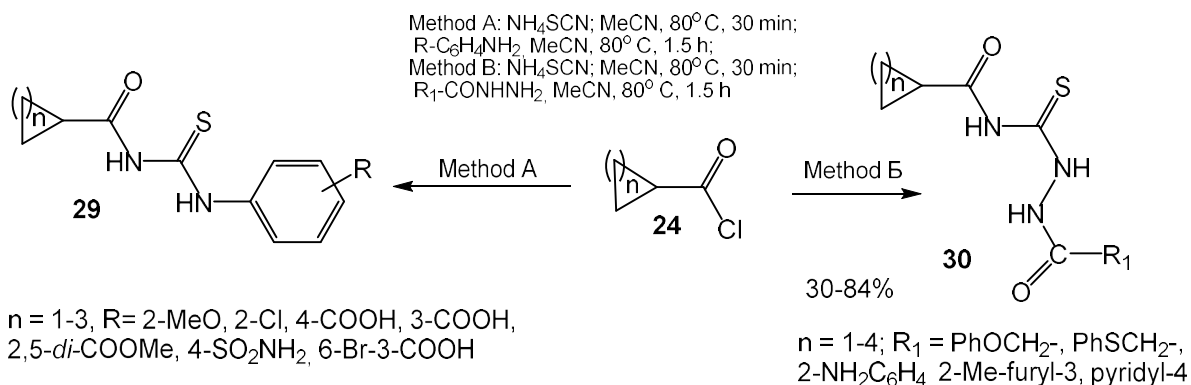
Fig. 9. “One-pot” synthesis of N -cycloalkylcarbonyl- N' -arylthioureas and N -cycloalkylcarbonyl- N' -acyl-(aroyl-, heteroyl-)thiosemicarbazides
