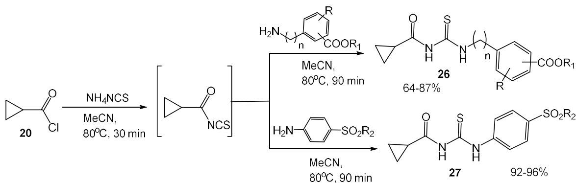
Fig. 7. “One-pot” synthesis of N -cycloalkylcarbonyl- N' -arylthioureas
