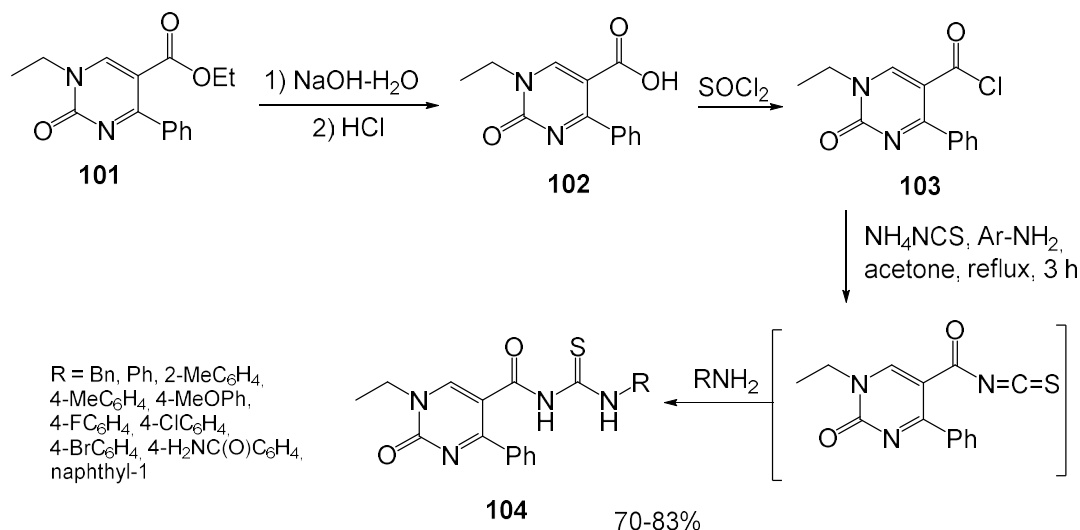
Fig. 28. Antitumor strategy among 1-ethyl-2-oxo-4-phenyl- N -(arylcabamothioyl)-1,2-dihydropyrimidine-5-carboxamides
